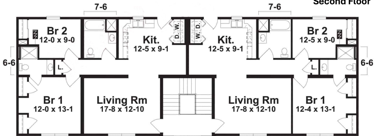
Second Floor
